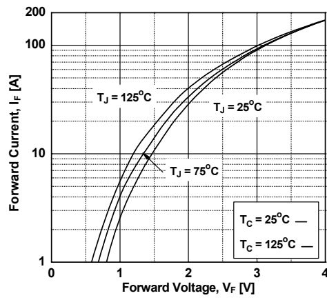
Figure 19. Forward Characteristics
