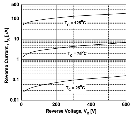
Figure 20. Reverse Current
